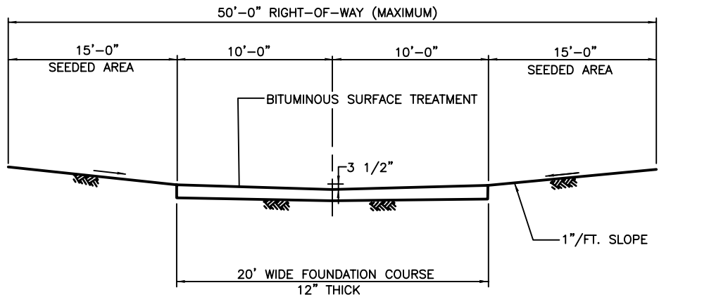
DEPRESSED ROADWAY
