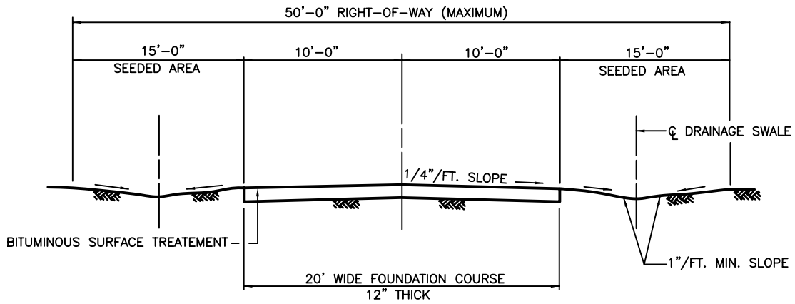
CROWNED ROADWAY
