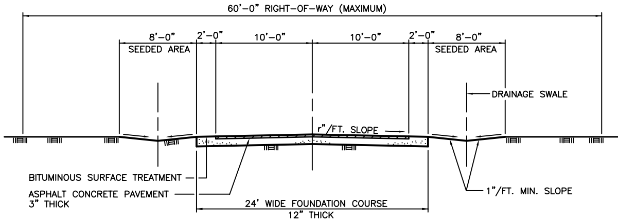
TYPICAL SECTION – ASPHALT CONCRETE PAVEMENT
