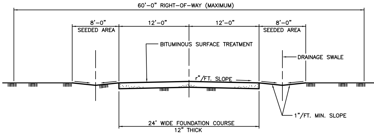
TYPICAL SECTION – SURFACE TREATMENT
